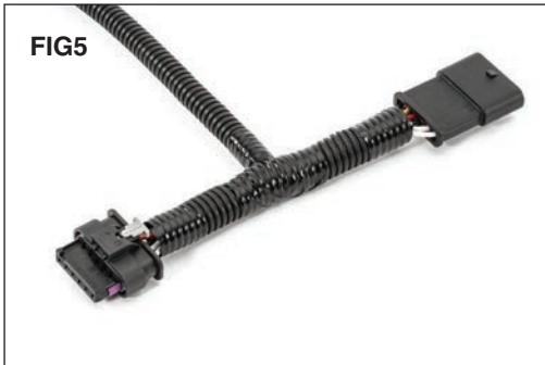
Locate the "T" end of the new light wiring harness.
