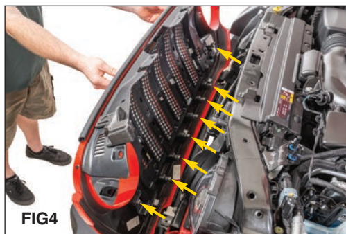
Gently tilt the grille forward and then gently pop the lower portion of grille from its (8) retaining clips. (FIG 4).
