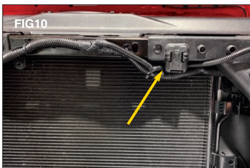
Note: The factory wiring harness will be routed behind the bracket as shown. (FIG 10)
