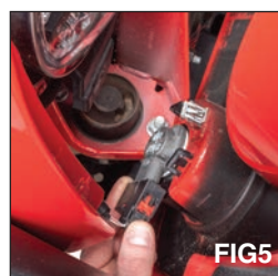
Disconnect the front turn signals by sliding the red locking tab backwards, depress the black latch and pull outward. (FIG 5)
