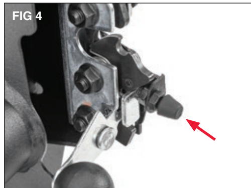
With a 10 mm wrench loosen the jam nuts on the door stop and thread the door stop in as far as it will go. (FIG4)
